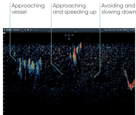
Sonar, Echogram, Classification example of Mackerel fishing, courtesy of F/V Gerda Marie
