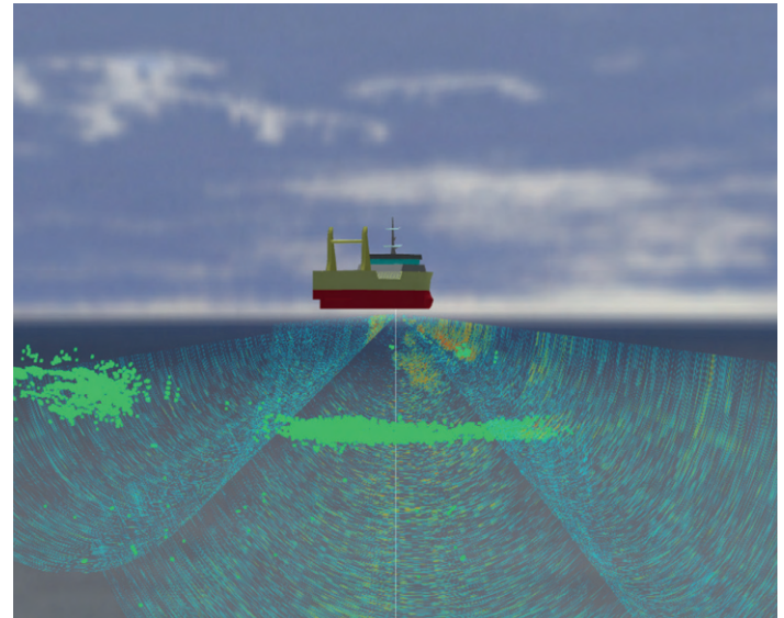
3D view, example of Mackerel fishing, courtesy of F/V Gerda Marie
